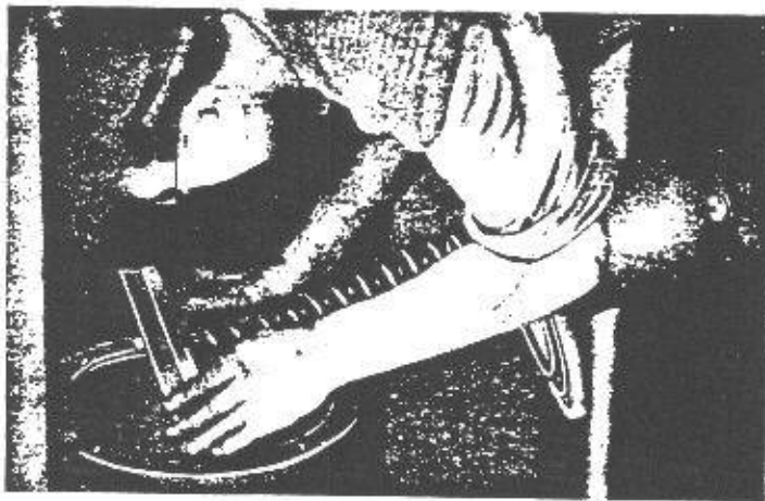
Illustration Showing Initial Step in Fitting Piston Packing Cup Into the Brake Cylinder
