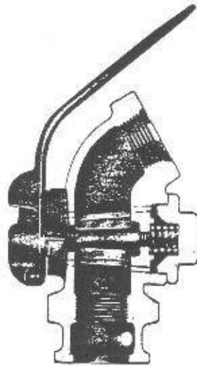
Fig. 19. End and Sectional Views of the Improved Angle Cock
